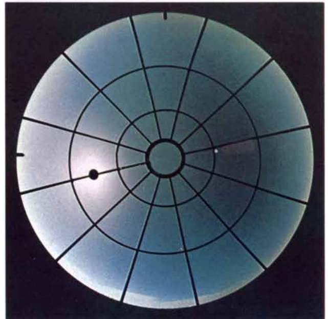
solar meridian. The axis of the polarizing filter was parallel to the solar meridian in all four photographs. At dawn maximum polarization ( dark region ), located 90 degrees from the sun, is centered in the sky. After sunrise the dark area shifts to the west. At the sun's maximum elevation in the southern sky the dark area shifts to the north; as the sun descends the dark area shifts around to the east. The two marks that appear on the horizon in the photograph indicate north and west.
