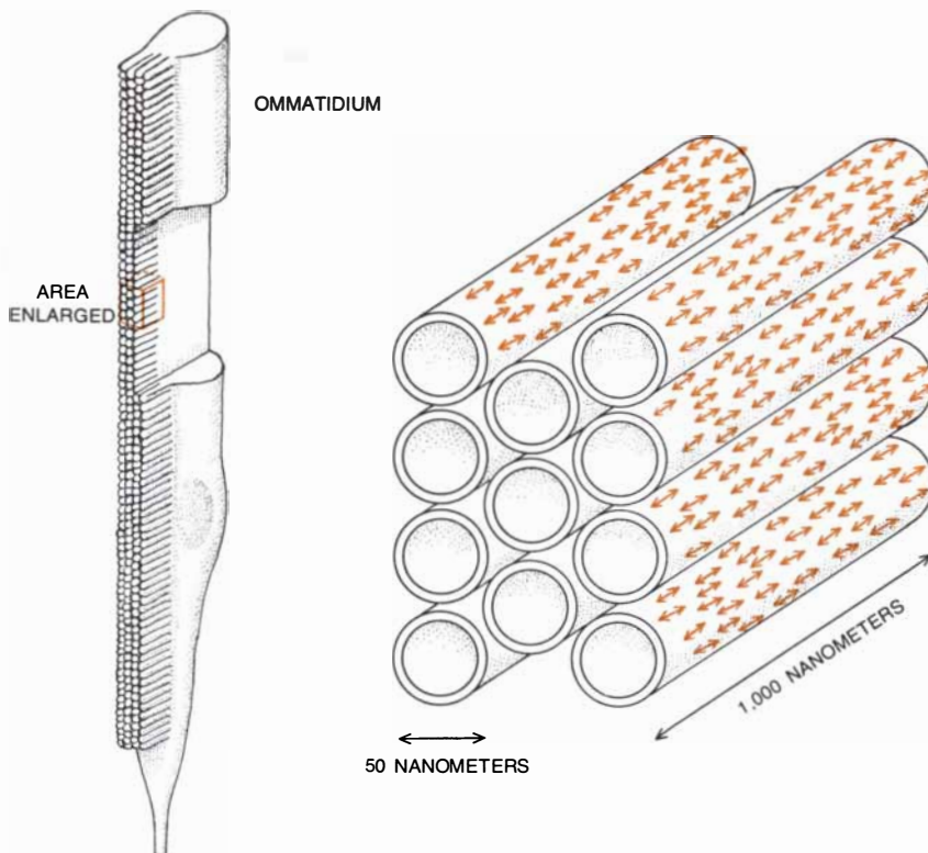
VISUAL CELLS of vertebrates ( top ) and invertebrates ( bottom ) differ in arrangement of photoreceptor membrane and orientation of molecules of visual pigment rhodopsin within membrane. In vertebrates axes of rhodopsin molecules ( color ) are randomly oriented; in insects they are parallel to long axis of tubelike microvilli. This maximizes absorption of polarized light.
