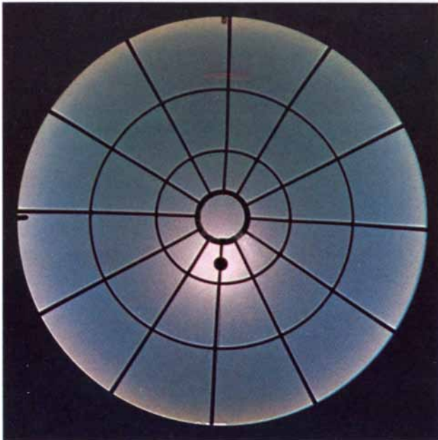
CHANGE IN THE POLARIZATION of the light of the sky at different times of the day is shown in this sequence of photographs made with a 180-degree "fish-eye" lens and a polarizing filter. The photographs, made on May 17, 1975, near Kairouan in Tunisia, were exposed at 5:15 A.M. ( top left ), 9:05 A.M. ( top right ), 12:30 P.M. ( bottom left ) and 3:40 P.M. ( bottom right ). A small black screen masks the sun in all the photographs but the first one; the screen also identifies the
