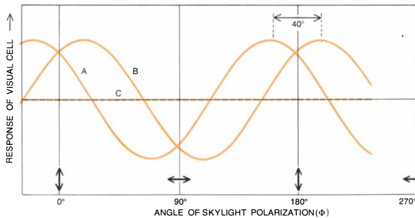
POLARIZATION-DETECTING SYSTEM of the honeybee is depicted schematically. The ultraviolet receptors of two adjacent ommatidia, one twisting clockwise and the other counterclockwise, are sufficient for the detection of any direction of polarization. Both ommatidia scan nearly the same small patch of the sky, less than five degrees in diameter. In the two ommatidia three types of ultraviolet receptors have to cooperate: polarization-insensitive cells (signal C) and two independent polarization-sensitive cells (signals A and B). This set of cells can unambiguously detect any direction of polarization ( \Phi ). The directions of maximum sensitivity of the two polarization-sensitive cells differ by about 40 degrees, as is shown by the curves at the right. The nerve fibers extending from the ultraviolet receptors extend through the first of the insect's two visual ganglia (the lamina) to the second (the medulla). The nerve fibers extending from the receptors sensitive to green and blue light rather than to ultraviolet end in lamina.
