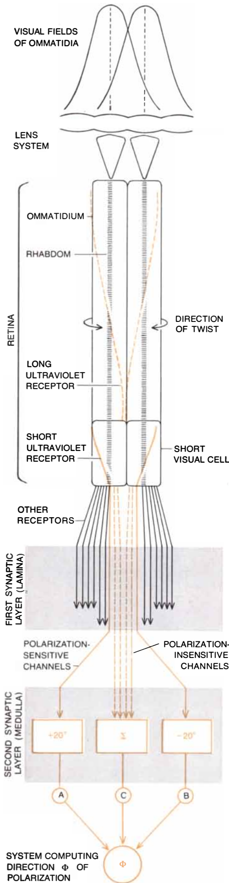
POLARIZATION-DETECTING SYSTEM of the honeybee is depicted schematically. The ultraviolet receptors of two adjacent ommatidia, one twisting clockwise and the other counterclockwise, are sufficient for the detection of any direction of polarization. Both ommatidia scan nearly the same small patch of the sky, less than five degrees in diameter. In the two ommatidia three types of ultraviolet receptors have to cooperate: polarization-insensitive cells (signal C) and two independent polarization-sensitive cells (signals A and B). This set of cells can unambiguously detect any direction of polarization ( \Phi ). The directions of maximum sensitivity of the two polarization-sensitive cells differ by about 40 degrees, as is shown by the curves at the right. The nerve fibers extending from the ultraviolet receptors extend through the first of the insect's two visual ganglia (the lamina) to the second (the medulla). The nerve fibers extending from the receptors sensitive to green and blue light rather than to ultraviolet end in lamina.
